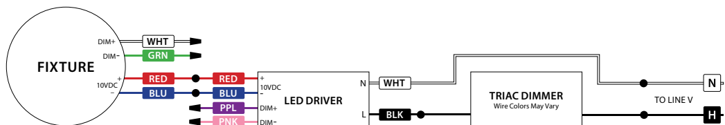
Forward Phase Dimming
