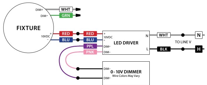
0 - 10 Volt Dimming (Alternate)
