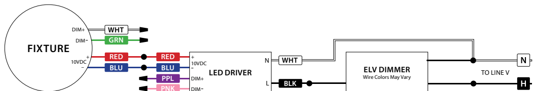
Reverse Phase Dimming
