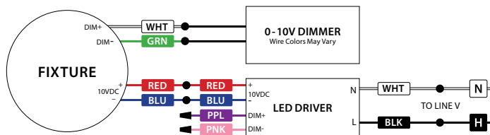
0 - 10 Volt Dimming (Preferred)
